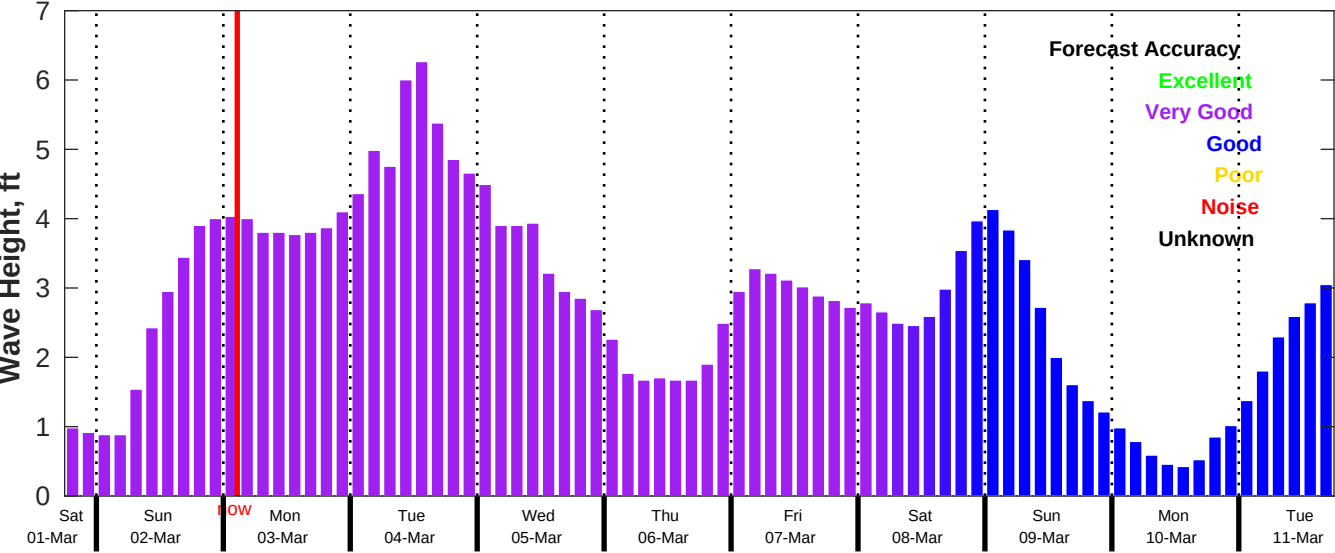
CMEMS Wave Forecast for NDBC 42035 from 01-Mar-2025 18:00:00 to 11-Mar-2025 18:00:00
