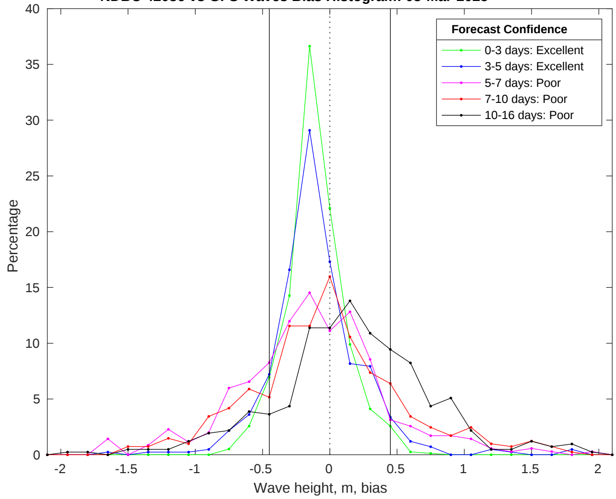
NDBC 42036 vs GFS Waves Bias Histogram: 03-Mar-2025
