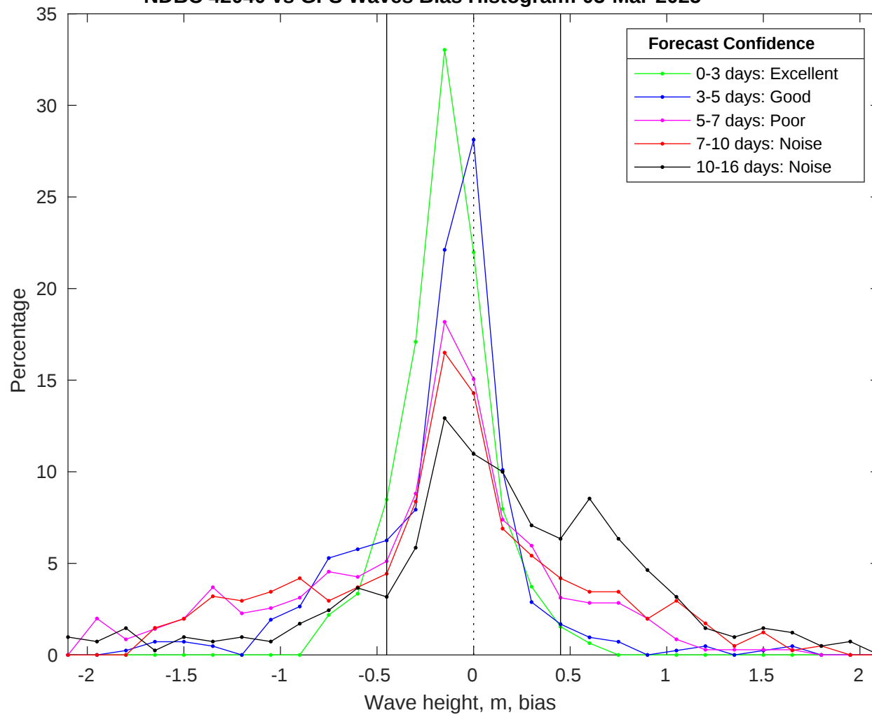
NDBC 42040 vs GFS Waves Bias Histogram: 03-Mar-2025
