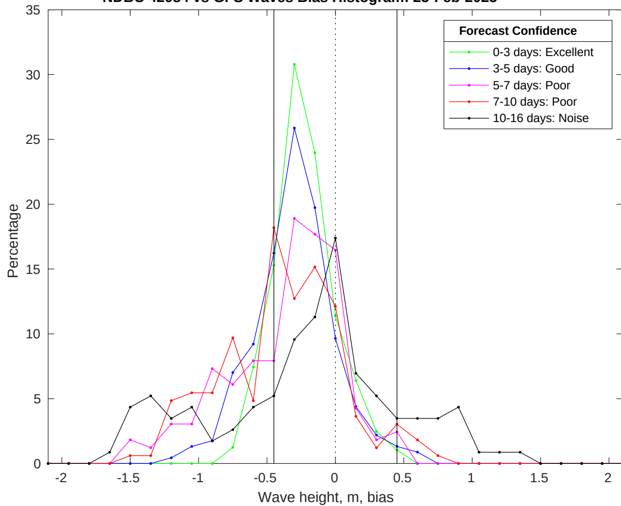
NDBC 42084 vs GFS Waves Bias Histogram: 25-Feb-2025
