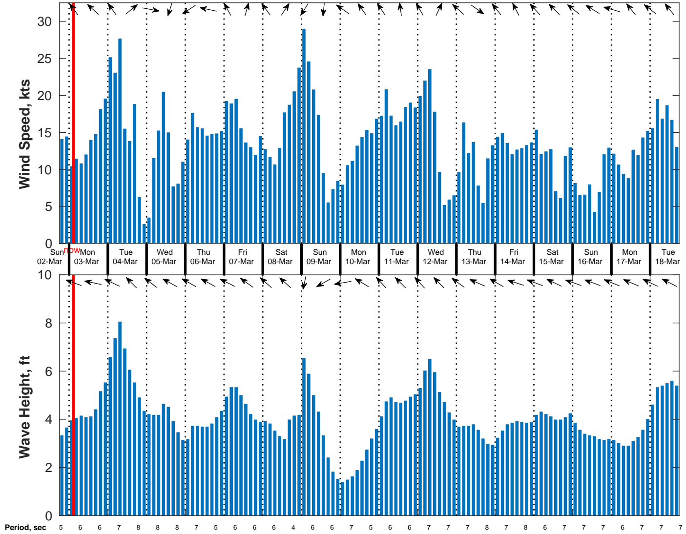
Wind & Wave Forecast for NDBC 42092 from 02-Mar-2025 18:00:00 to 18-Mar-2025 18:00:00
