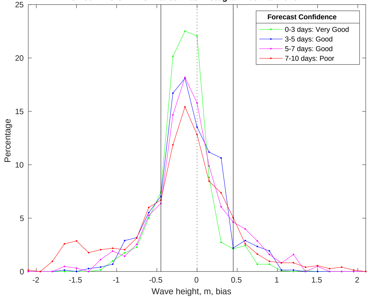
NDBC 46011 vs CMEMS Waves Bias Histogram: 03-Mar-2025
