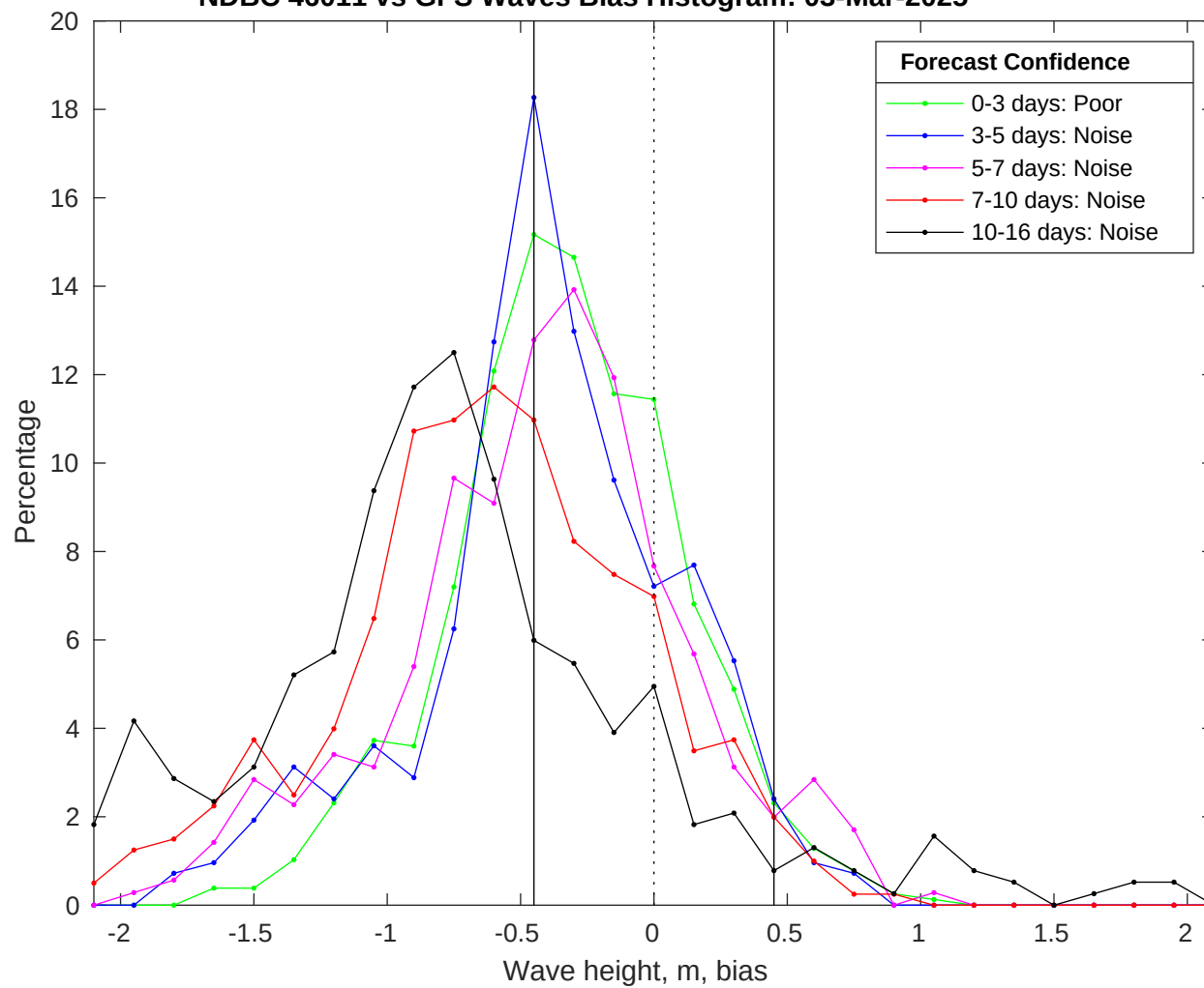
NDBC 46011 vs GFS Waves Bias Histogram: 03-Mar-2025
