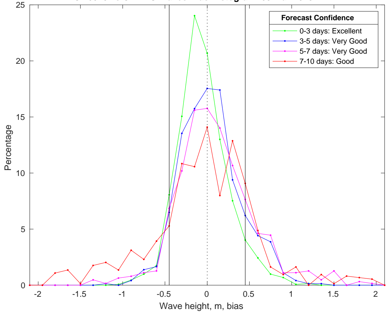
NDBC 46028 vs CMEMS Waves Bias Histogram: 03-Mar-2025
