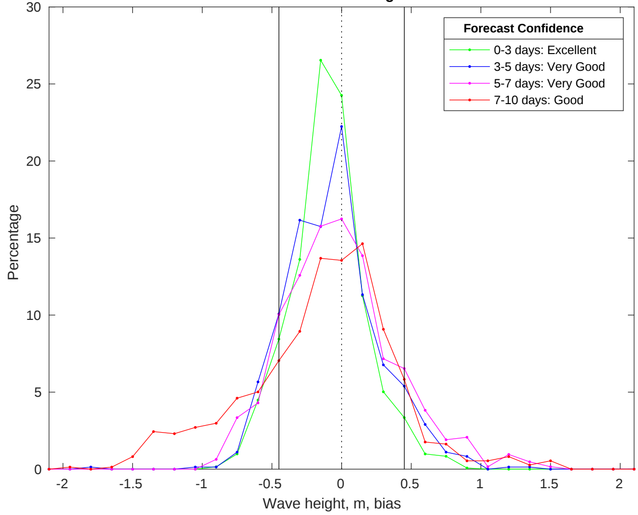
NDBC 46054 vs CMEMS Waves Bias Histogram: 03-Mar-2025
