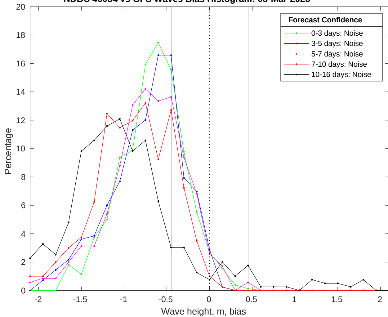
NDBC 46054 vs GFS Waves Bias Histogram: 03-Mar-2025
