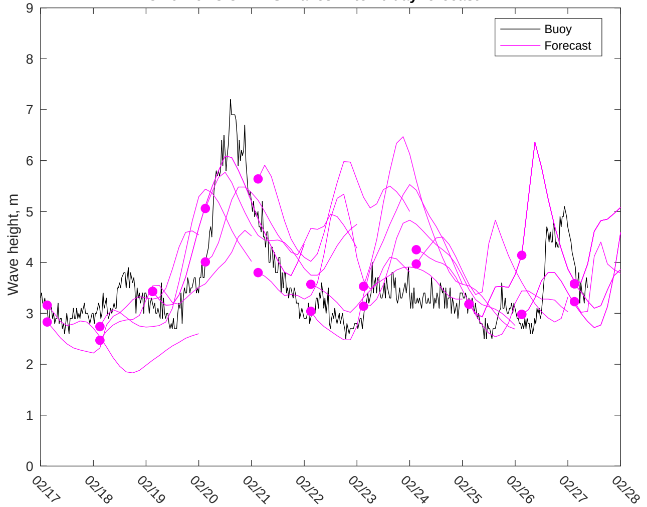
NDBC 46246 vs CMEMS Waves: 7 to 10 day forecast
