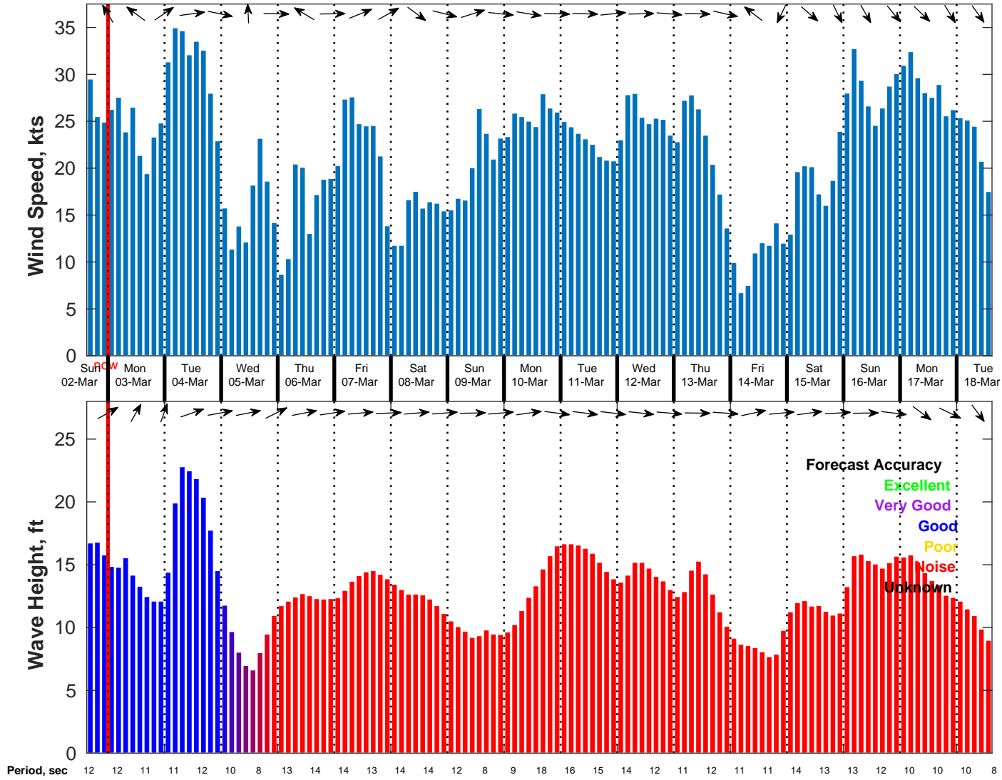
Wind & Wave Forecast for NDBC 46246 from 02-Mar-2025 15:00:00 to 18-Mar-2025 15:00:00
