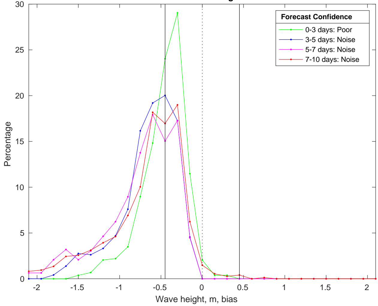
NDBC 51209 vs CMEMS Waves Bias Histogram: 03-Mar-2025
