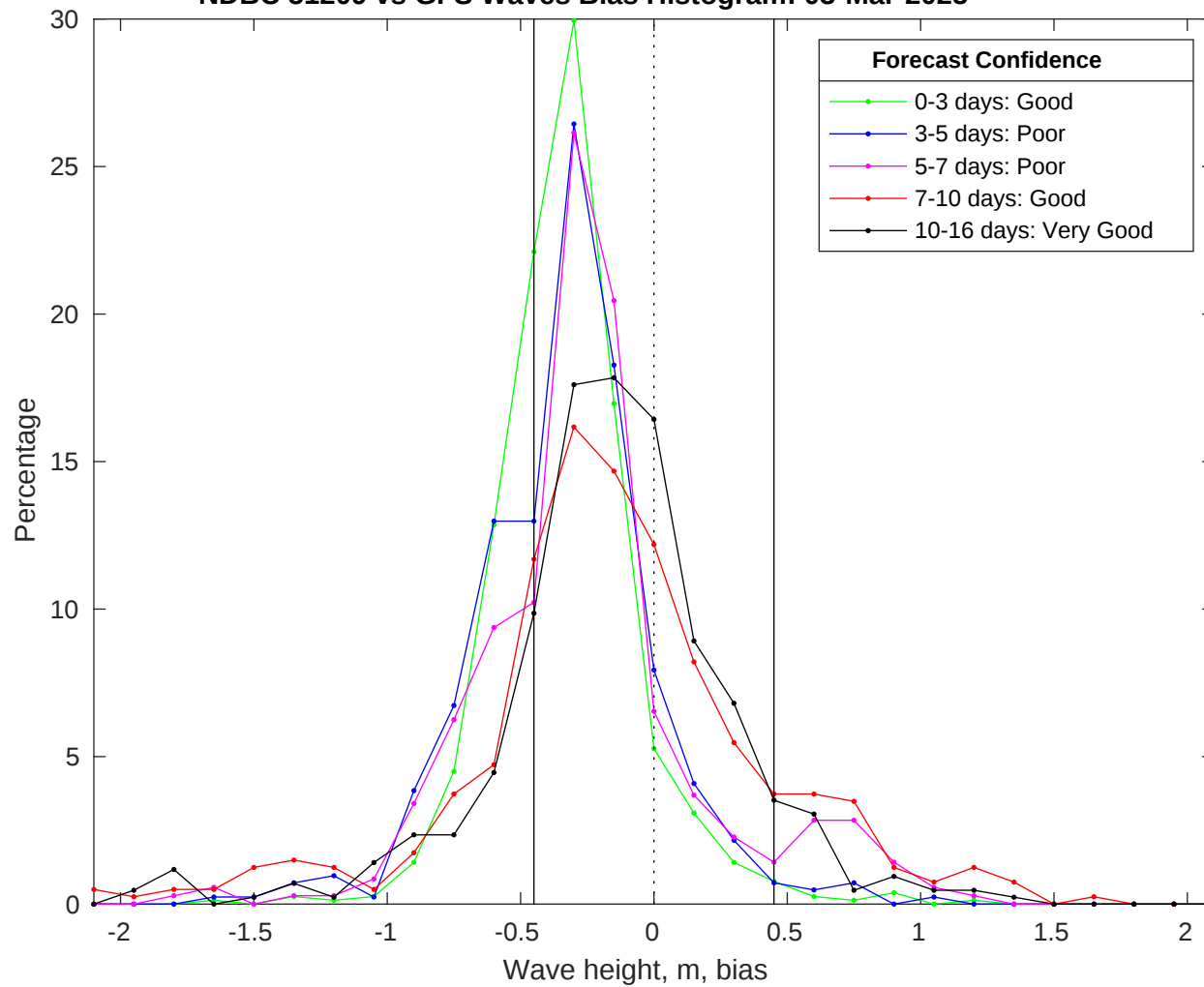
NDBC 51209 vs GFS Waves Bias Histogram: 03-Mar-2025
