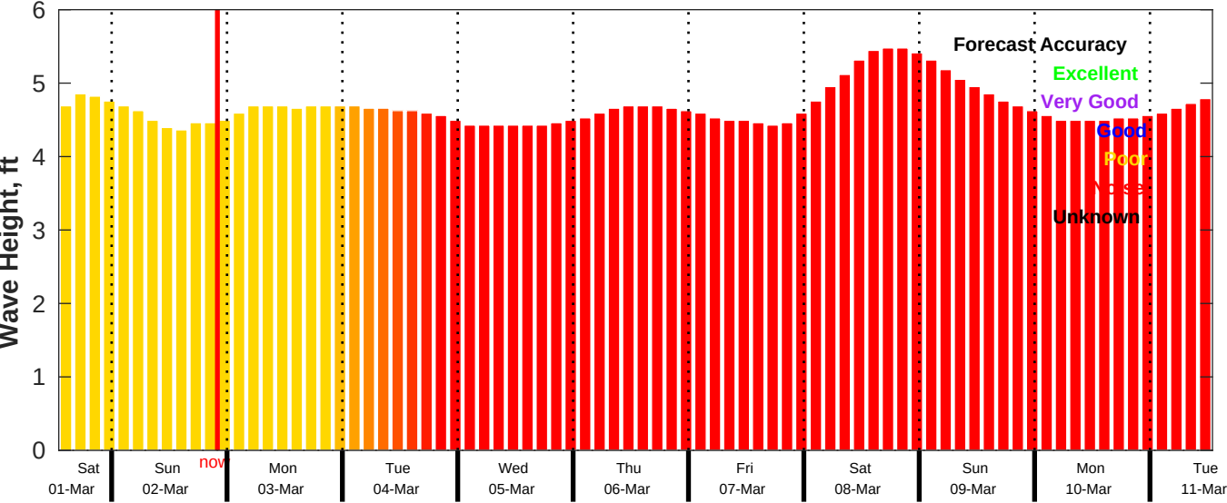
CMEMS Wave Forecast for NDBC 51209 from 01-Mar-2025 13:00:00 to 11-Mar-2025 13:00:00
