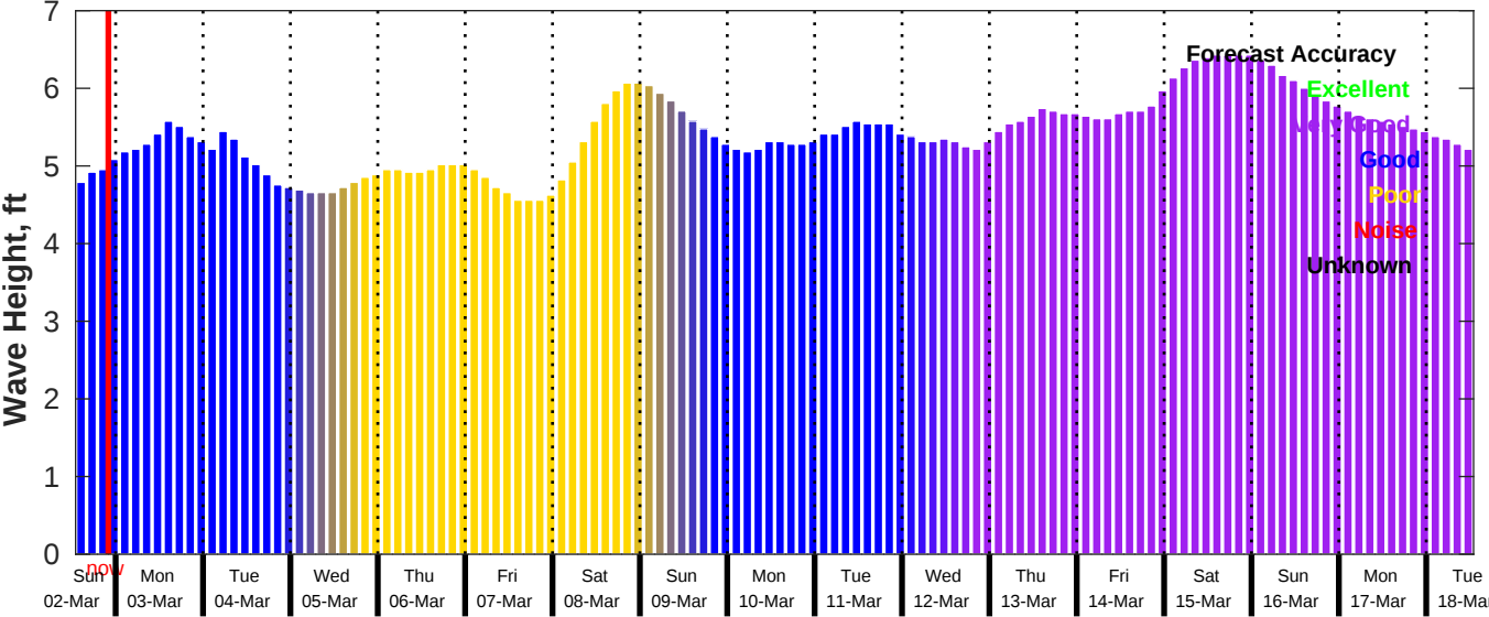
GFS Wave Forecast for NDBC 51209 from 02-Mar-2025 13:00:00 to 18-Mar-2025 13:00:00
