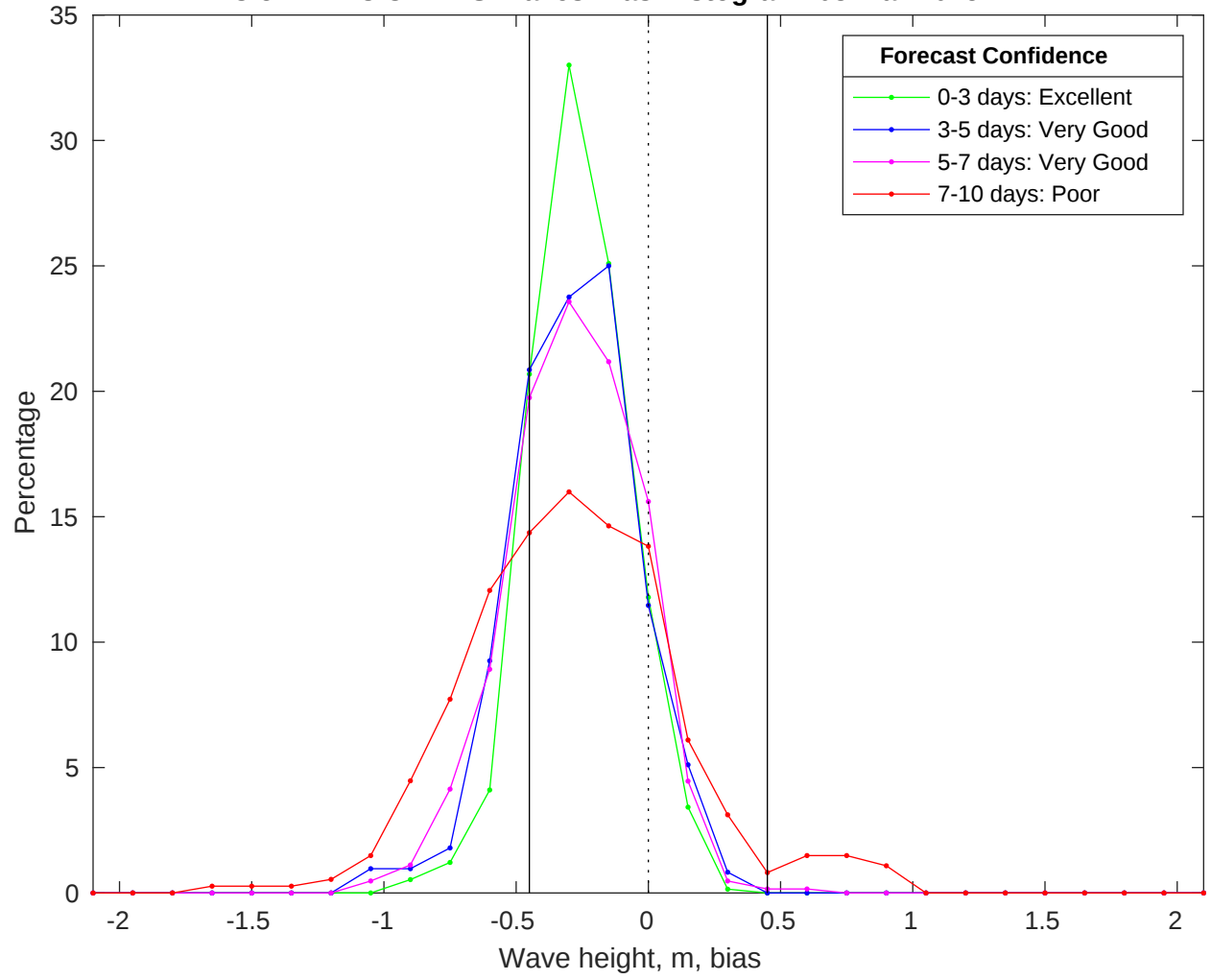
NDBC 52211 vs CMEMS Waves Bias Histogram: 03-Mar-2025
