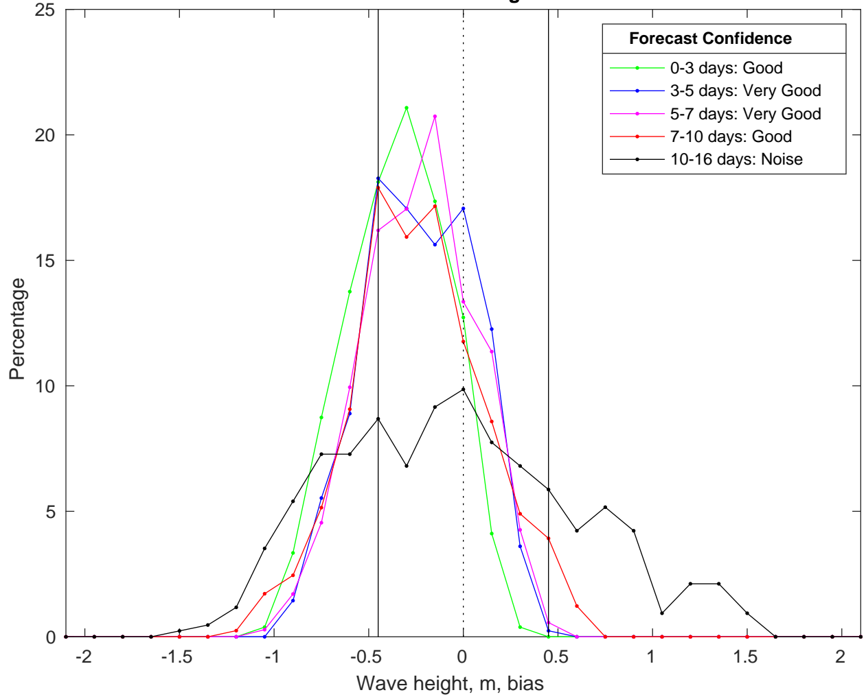
NDBC 52211 vs GFS Waves Bias Histogram: 03-Mar-2025
