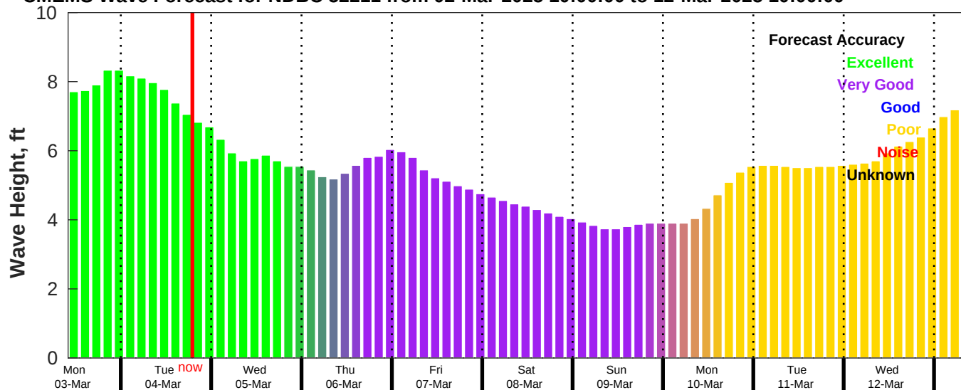
CMEMS Wave Forecast for NDBC 52211 from 02-Mar-2025 10:00:00 to 12-Mar-2025 10:00:00
