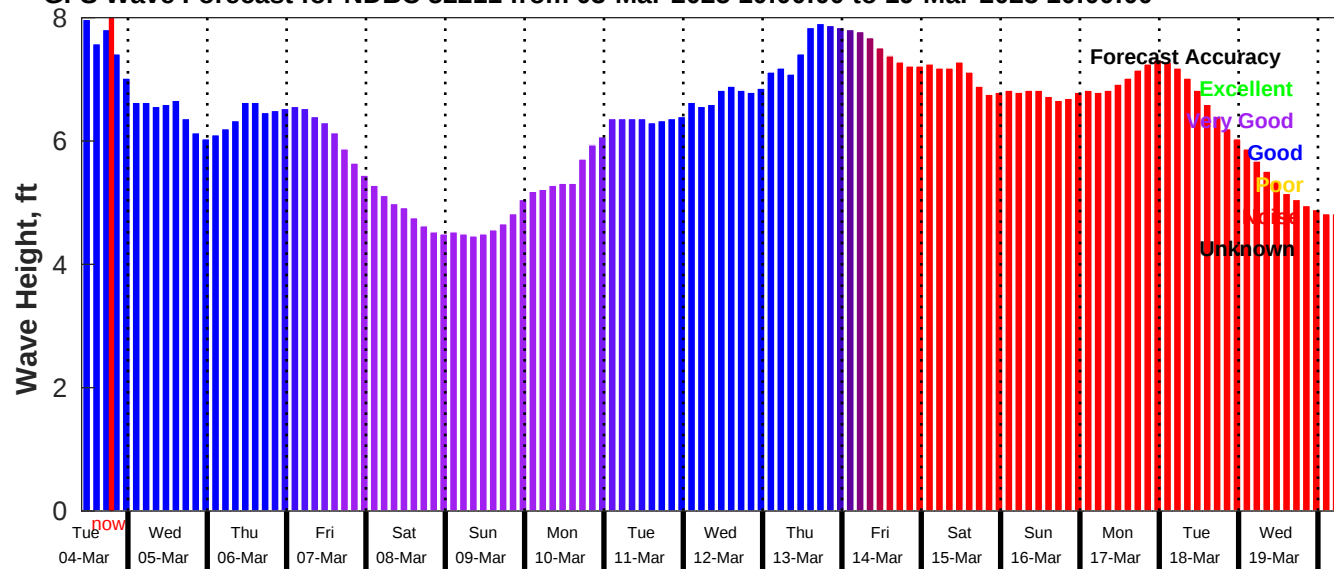
GFS Wave Forecast for NDBC 52211 from 03-Mar-2025 10:00:00 to 19-Mar-2025 10:00:00
