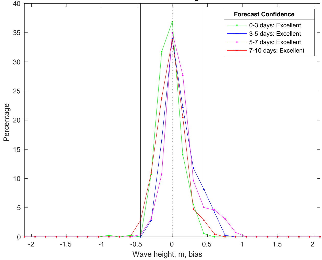
NDBC 52212 vs CMEMS Waves Bias Histogram: 03-Mar-2025
