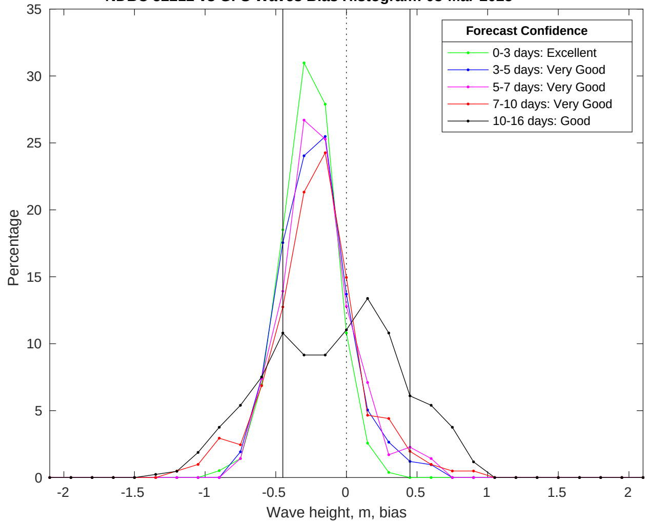
NDBC 52212 vs GFS Waves Bias Histogram: 03-Mar-2025
