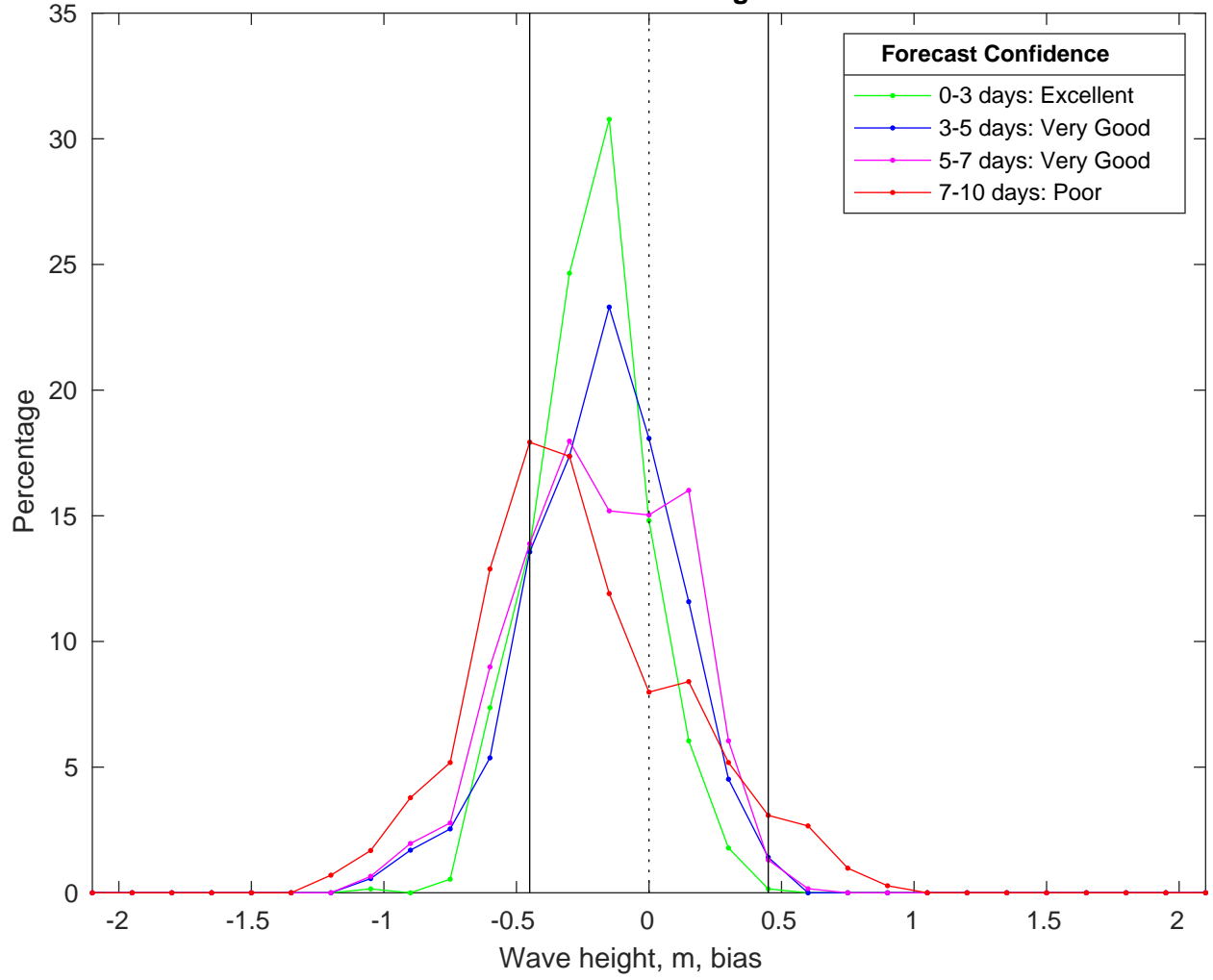
NDBC 52213 vs CMEMS Waves Bias Histogram: 03-Mar-2025
