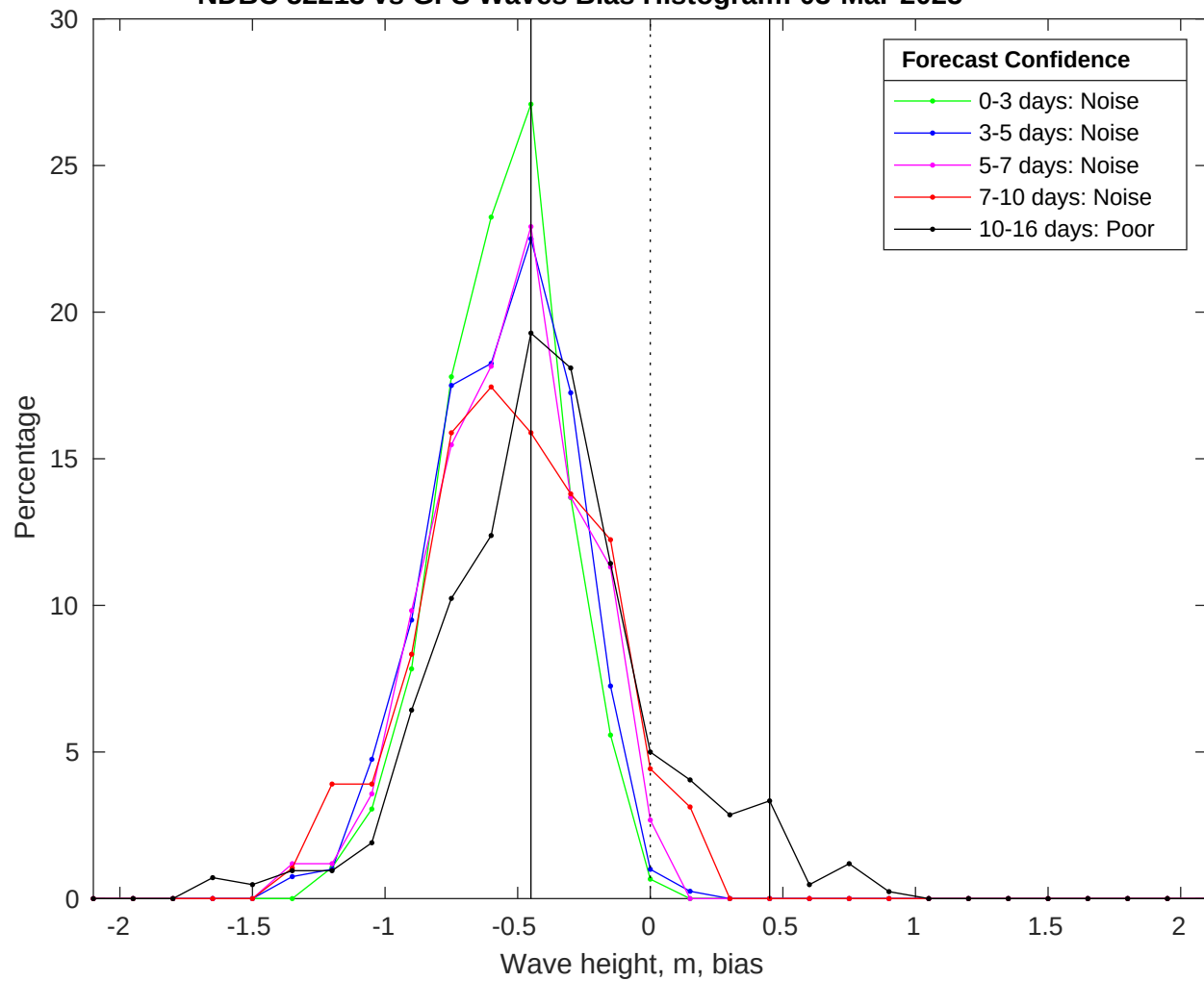
NDBC 52213 vs GFS Waves Bias Histogram: 03-Mar-2025
