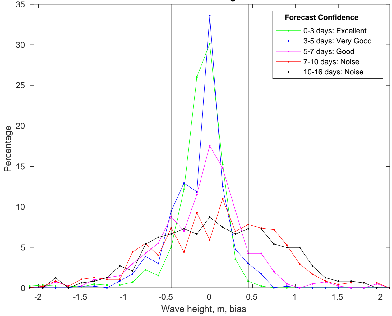
NDBC 41004 vs GFS Waves Bias Histogram: 04-Mar-2025
