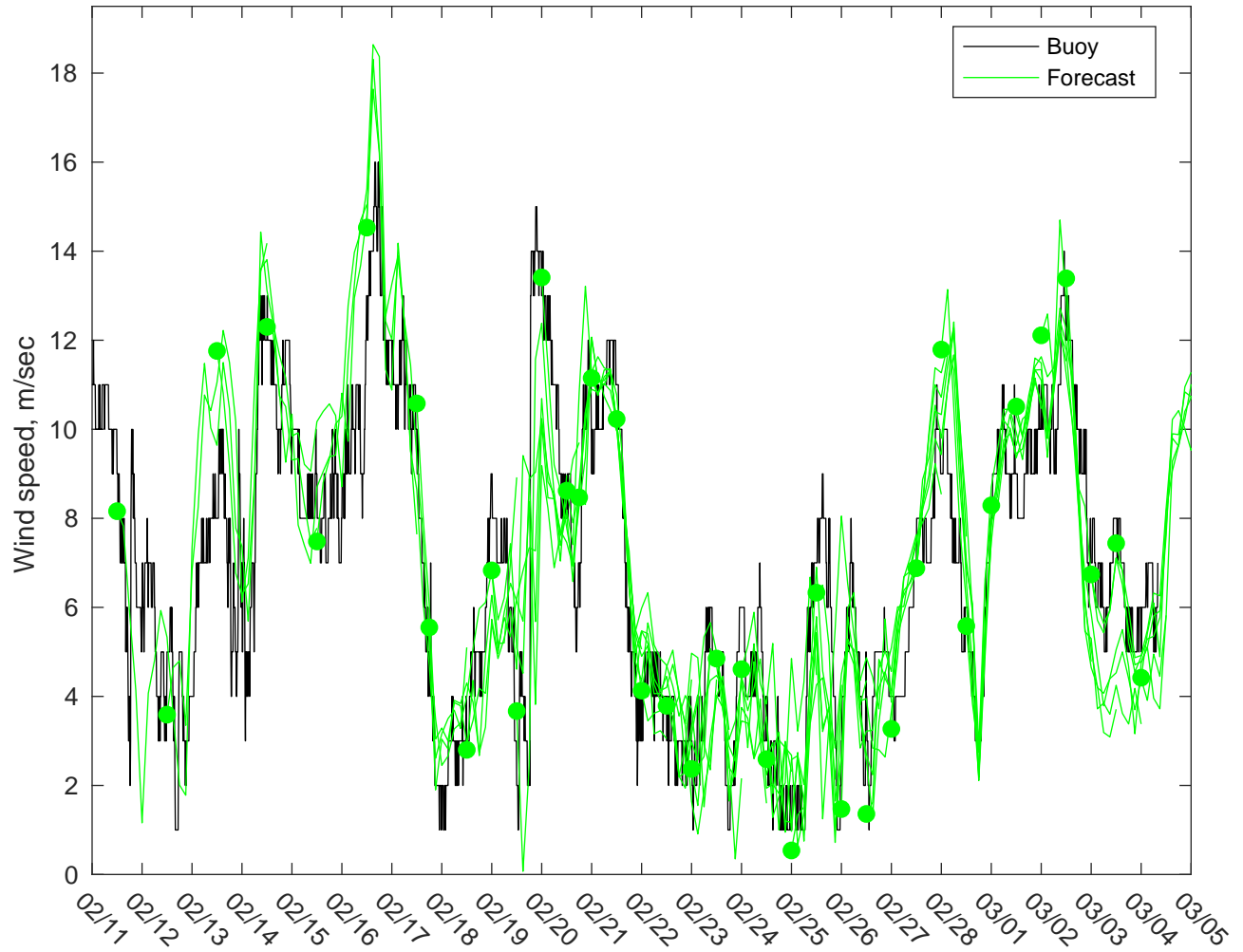
NDBC 41004 vs GFS Winds: 0 to 3 day forecast
