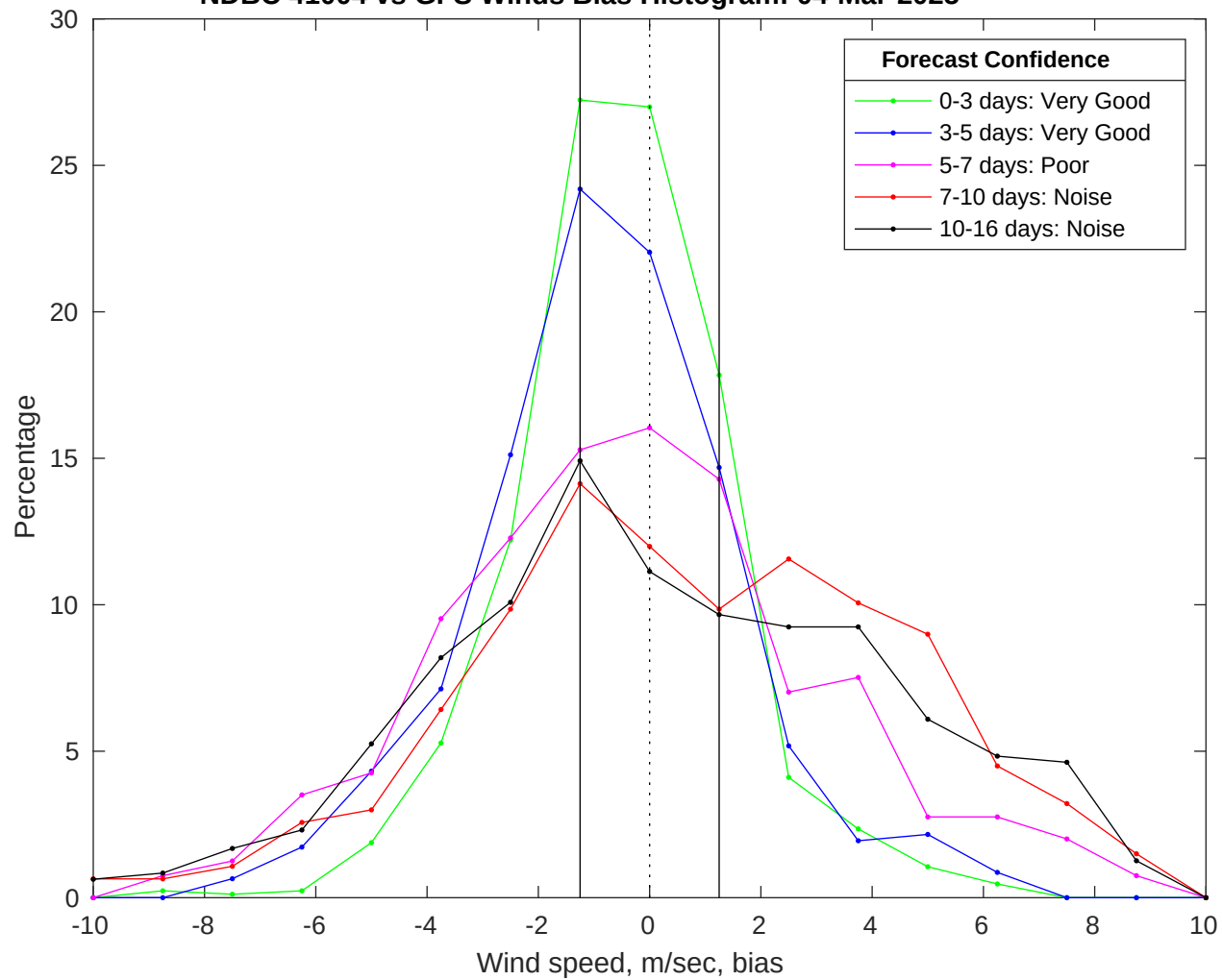
NDBC 41004 vs GFS Winds Bias Histogram: 04-Mar-2025
