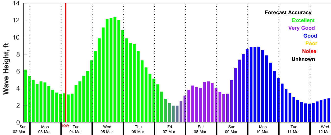
CMEMS Wave Forecast for NDBC 41004 from 02-Mar-2025 19:00:00 to 12-Mar-2025 19:00:00
