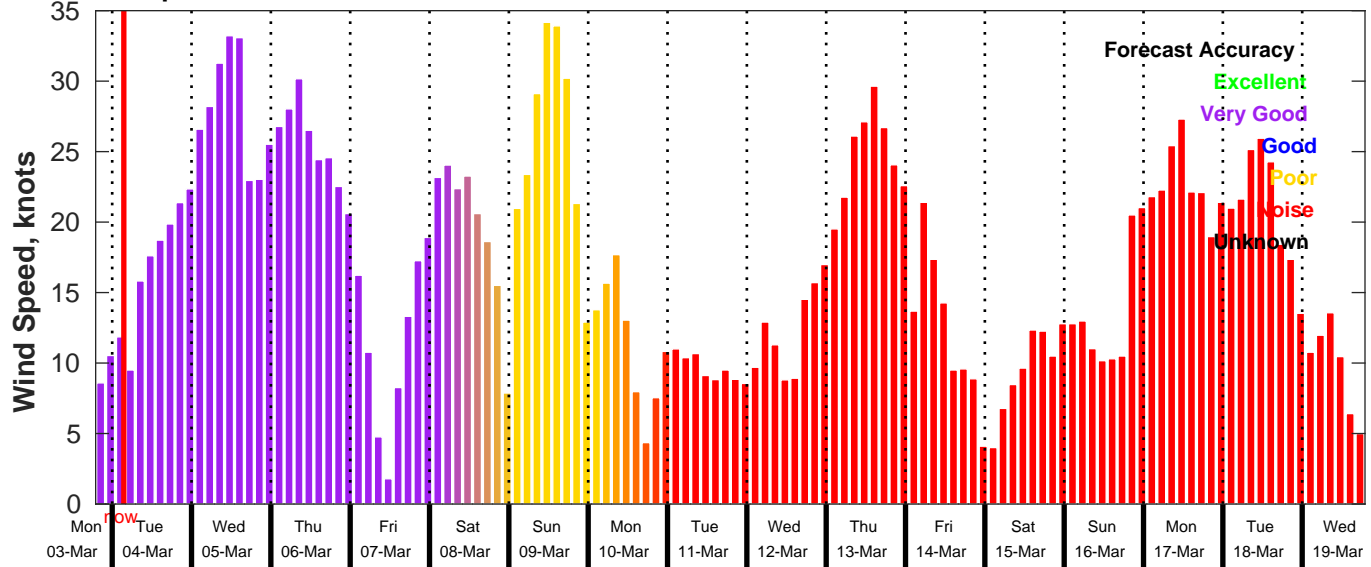
GFS Wind Speed Forecast for NDBC 41004 from 03-Mar-2025 19:00:00 to 19-Mar-2025 19:00:00
