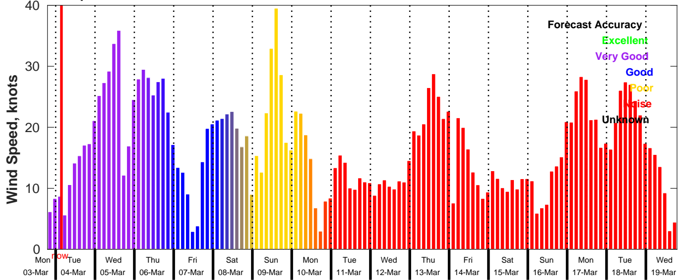
GFS Wind Speed Forecast for NDBC 41013 from 03-Mar-2025 19:00:00 to 19-Mar-2025 19:00:00
