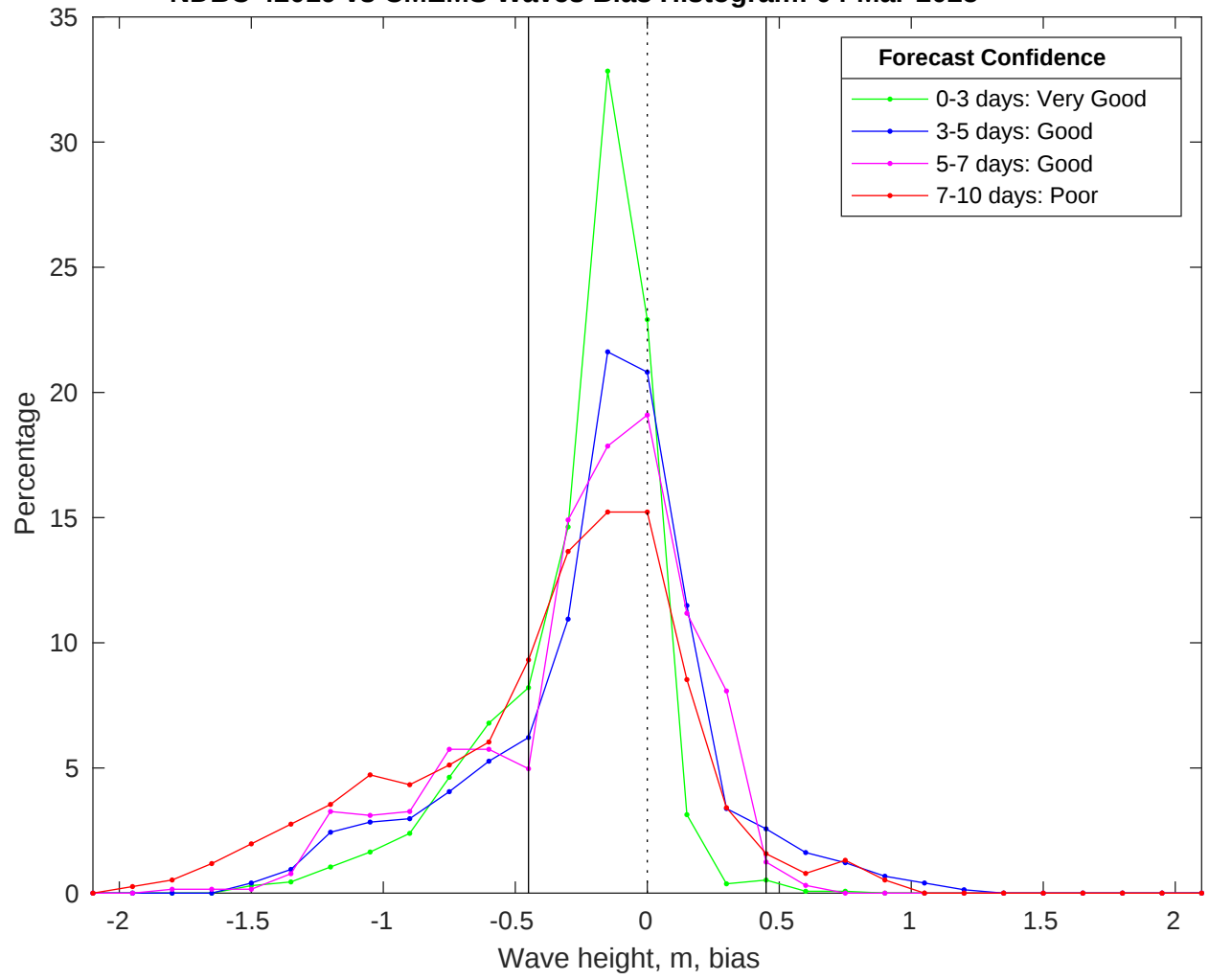
NDBC 42019 vs CMEMS Waves Bias Histogram: 04-Mar-2025
