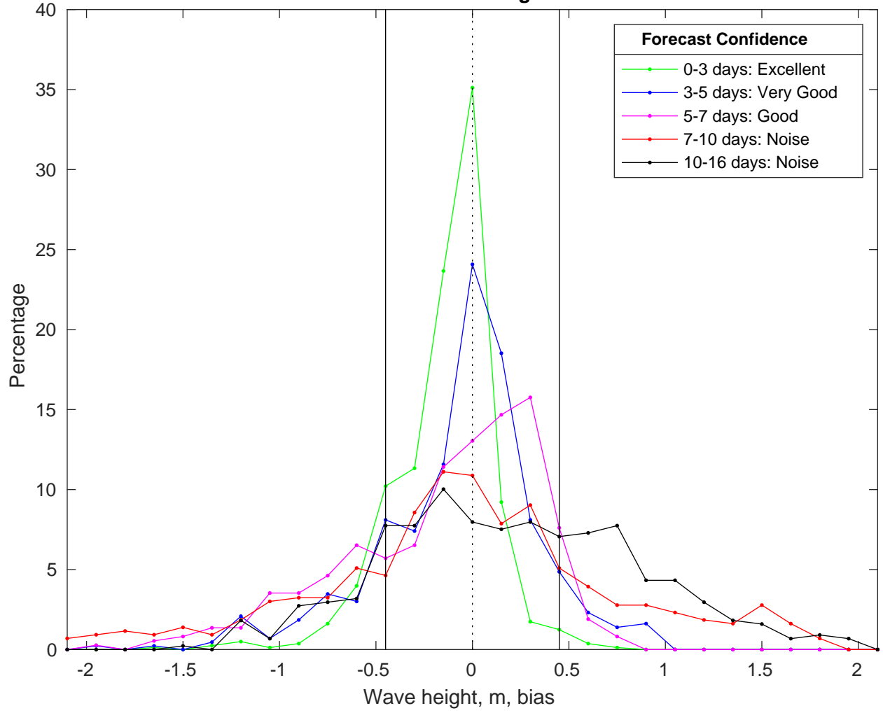
NDBC 42019 vs GFS Waves Bias Histogram: 04-Mar-2025
