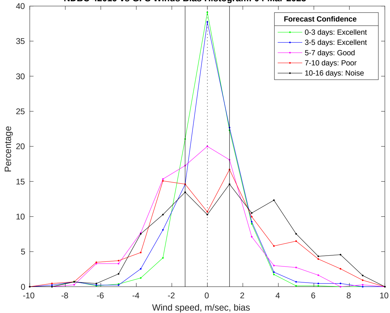
NDBC 42019 vs GFS Winds Bias Histogram: 04-Mar-2025
