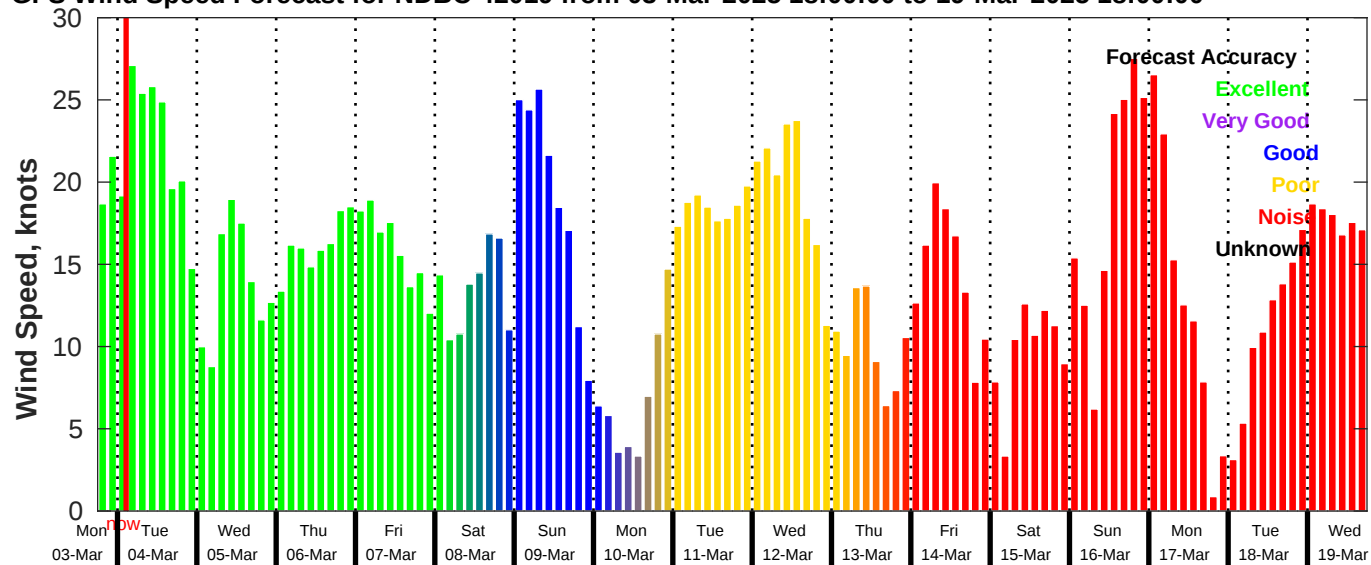
GFS Wind Speed Forecast for NDBC 42019 from 03-Mar-2025 18:00:00 to 19-Mar-2025 18:00:00
