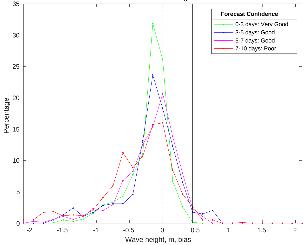
NDBC 42020 vs CMEMS Waves Bias Histogram: 04-Mar-2025
