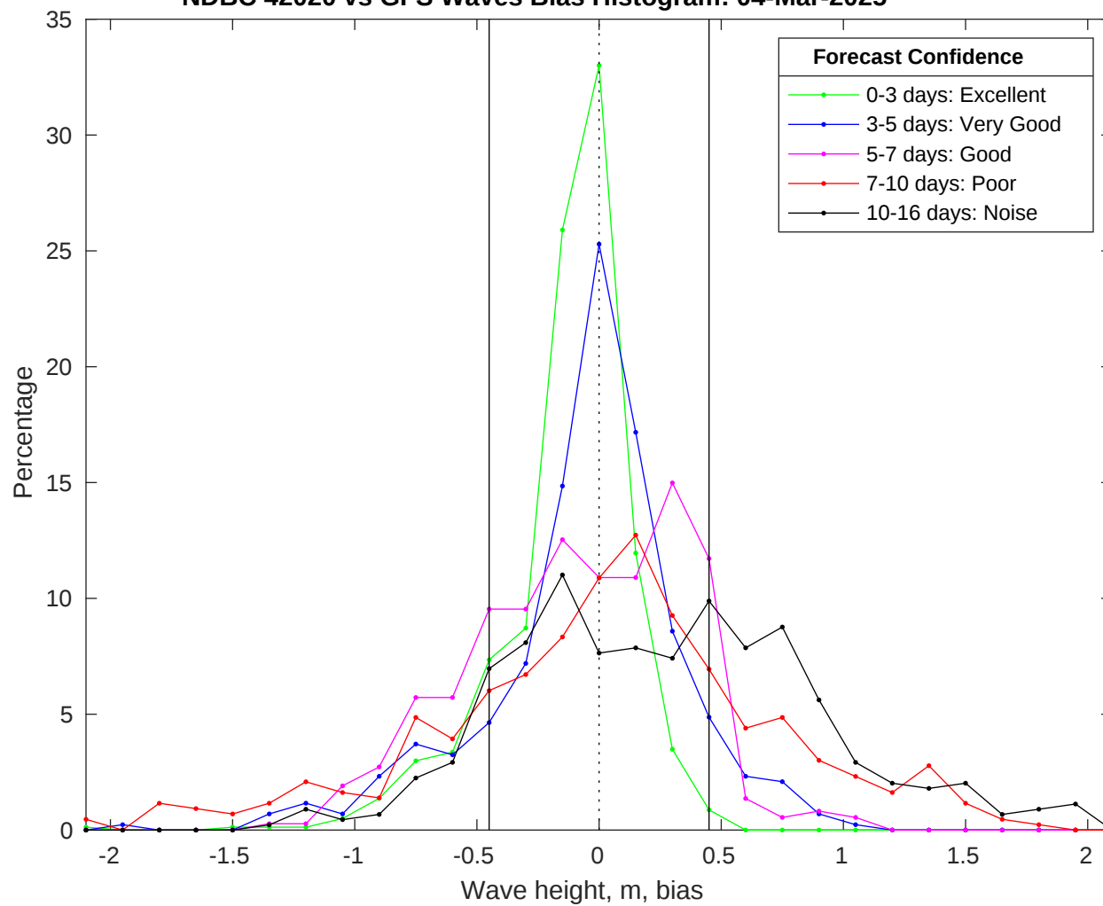
NDBC 42020 vs GFS Waves Bias Histogram: 04-Mar-2025
