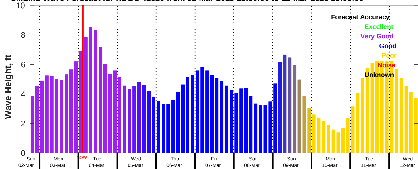
CMEMS Wave Forecast for NDBC 42020 from 02-Mar-2025 18:00:00 to 12-Mar-2025 18:00:00
