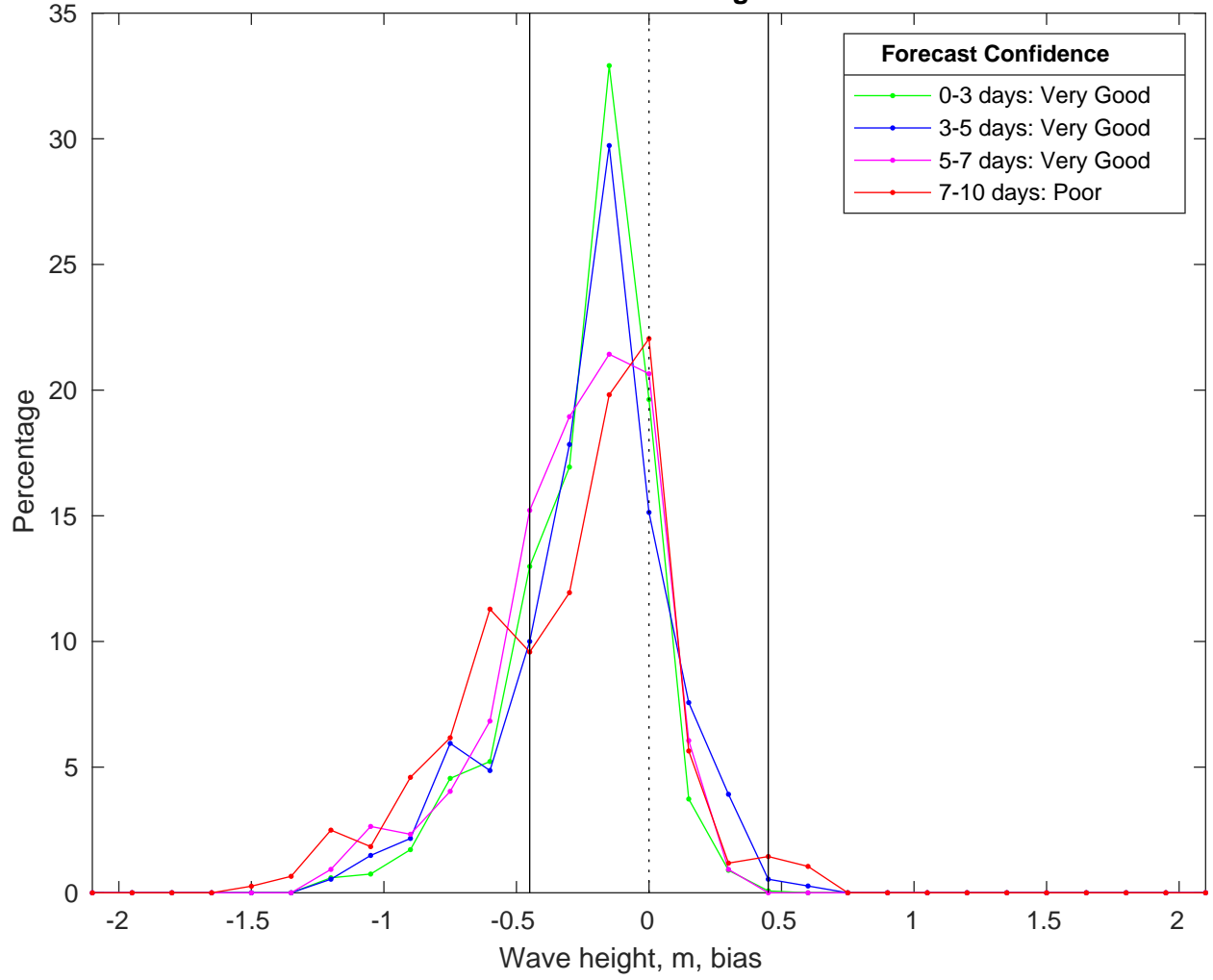
NDBC 42035 vs CMEMS Waves Bias Histogram: 04-Mar-2025
