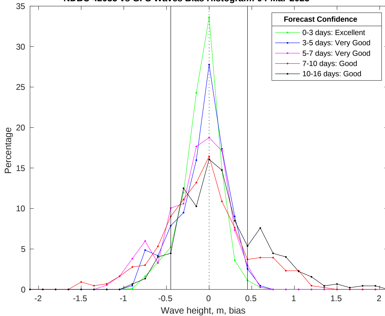
NDBC 42035 vs GFS Waves Bias Histogram: 04-Mar-2025
