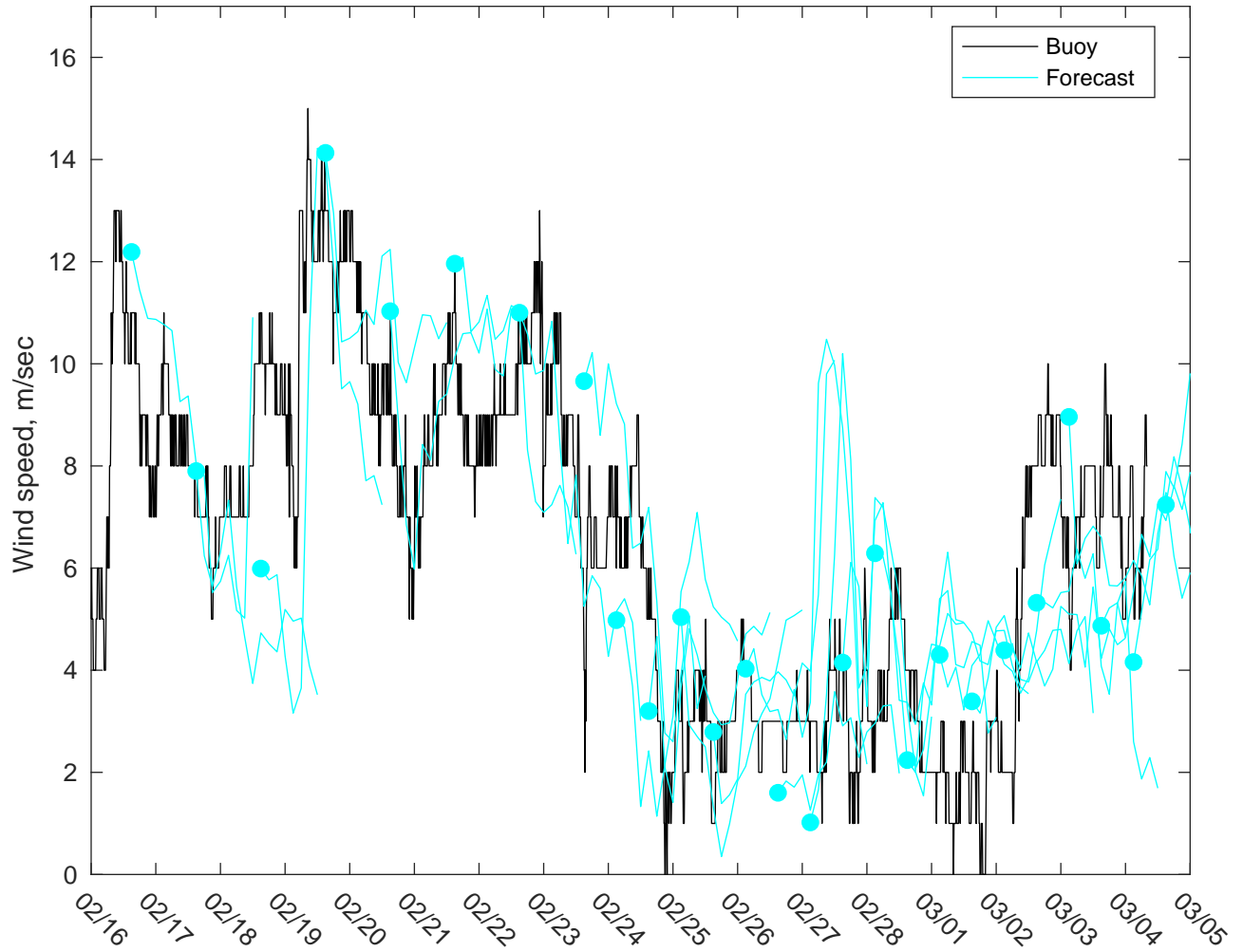
NDBC 42035 vs GFS Winds: 5 to 7 day forecast
