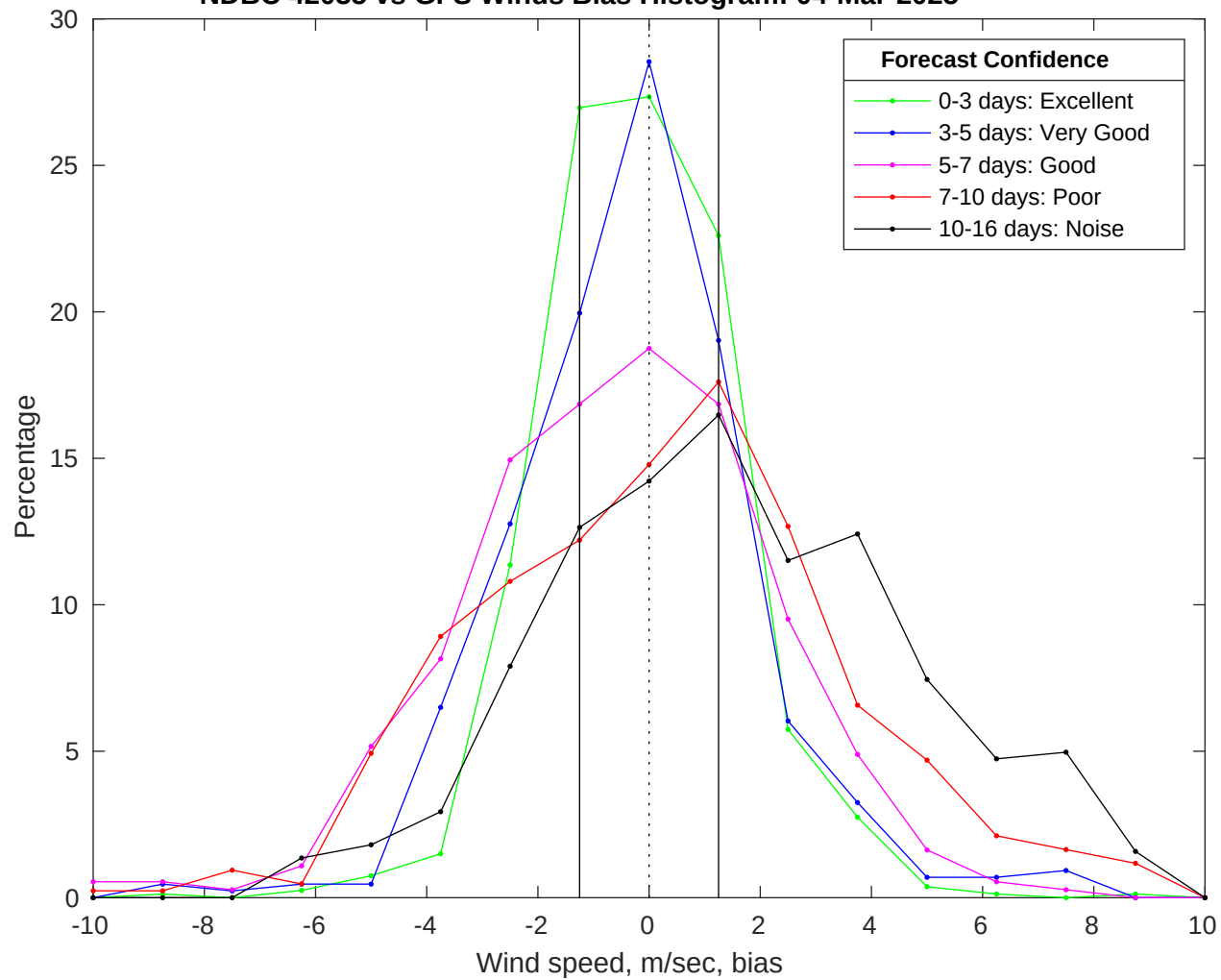
NDBC 42035 vs GFS Winds Bias Histogram: 04-Mar-2025
