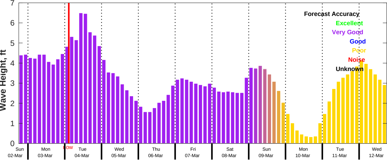
CMEMS Wave Forecast for NDBC 42035 from 02-Mar-2025 18:00:00 to 12-Mar-2025 18:00:00
