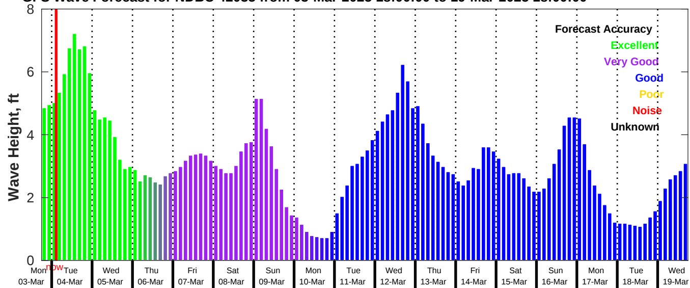
GFS Wave Forecast for NDBC 42035 from 03-Mar-2025 18:00:00 to 19-Mar-2025 18:00:00
