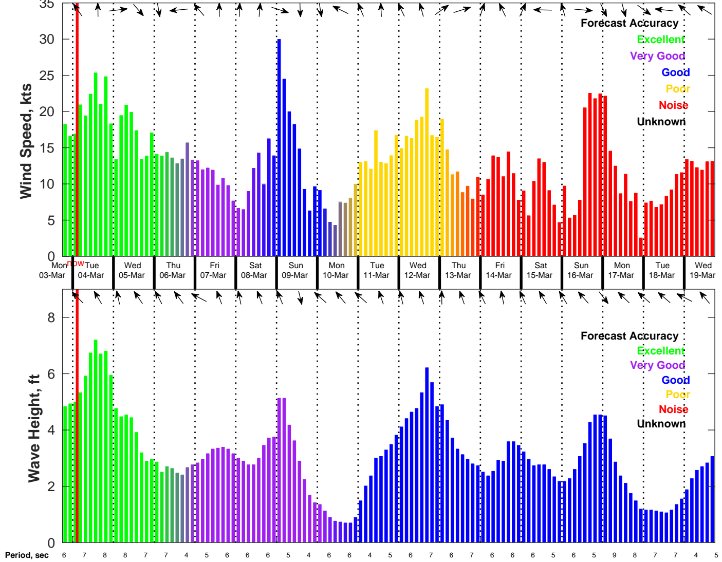
Wind & Wave Forecast for NDBC 42035 from 03-Mar-2025 18:00:00 to 19-Mar-2025 18:00:00
