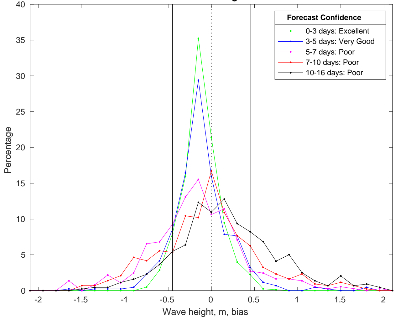
NDBC 42036 vs GFS Waves Bias Histogram: 04-Mar-2025
