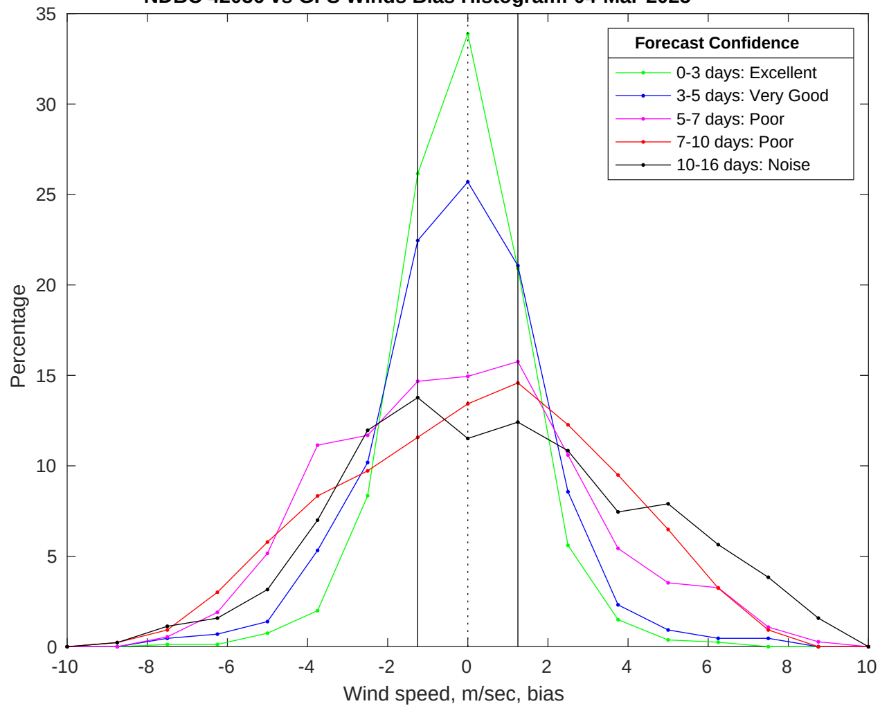
NDBC 42036 vs GFS Winds Bias Histogram: 04-Mar-2025
