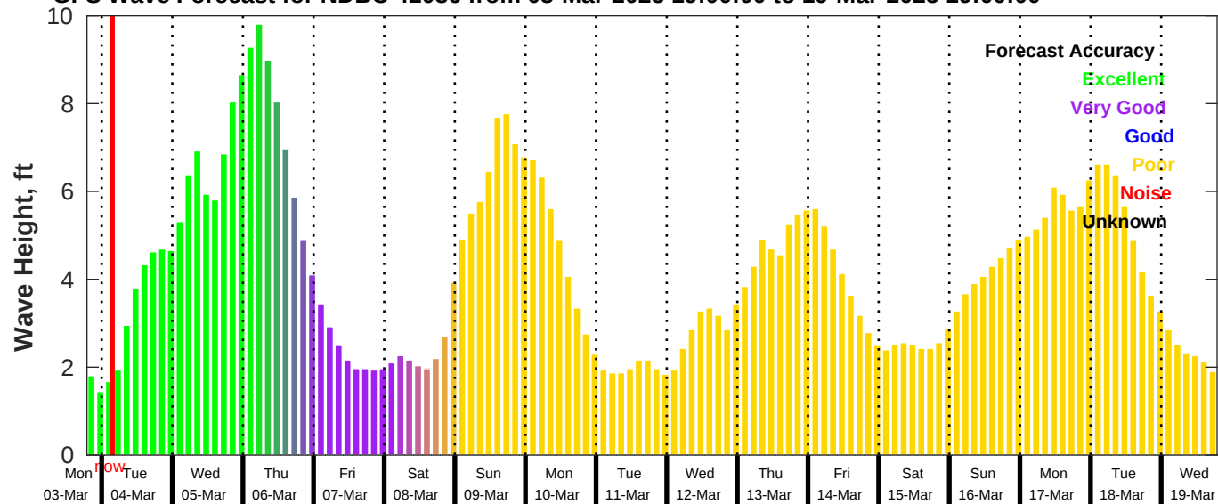
GFS Wave Forecast for NDBC 42036 from 03-Mar-2025 19:00:00 to 19-Mar-2025 19:00:00
