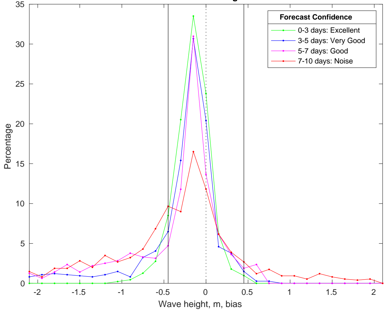
NDBC 42040 vs CMEMS Waves Bias Histogram: 04-Mar-2025
