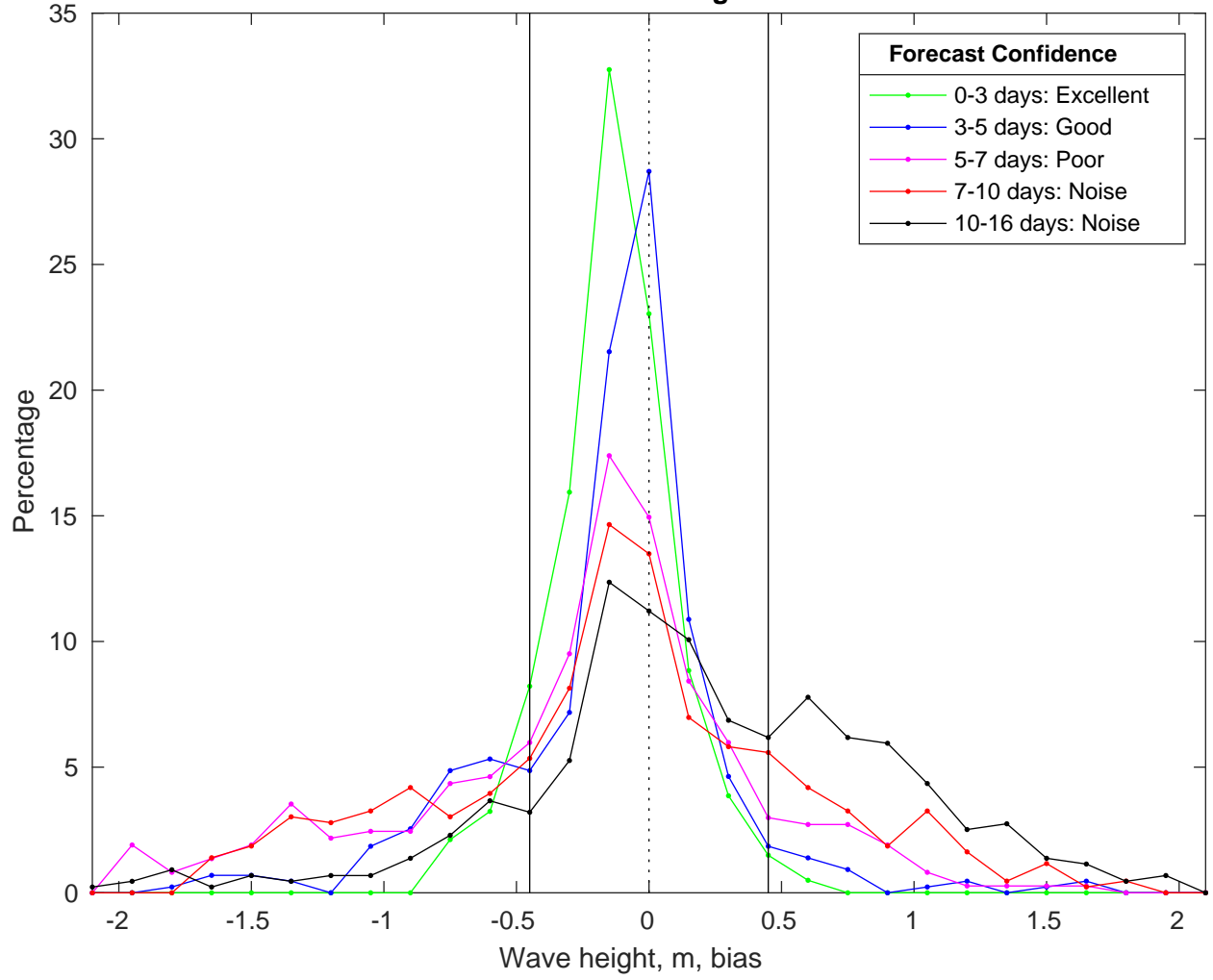
NDBC 42040 vs GFS Waves Bias Histogram: 04-Mar-2025
