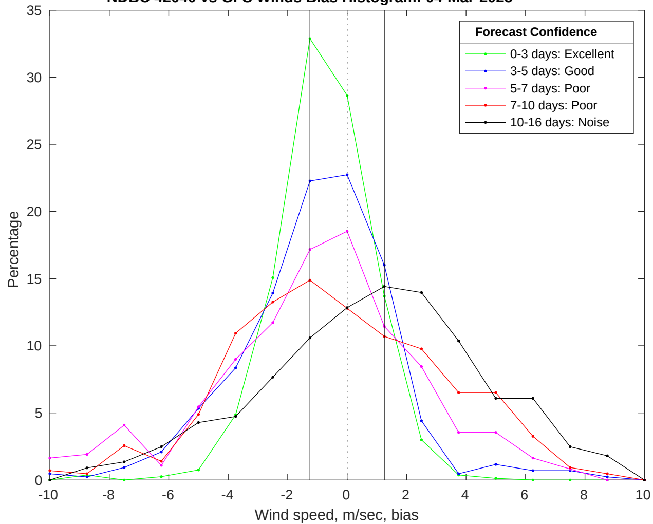
NDBC 42040 vs GFS Winds Bias Histogram: 04-Mar-2025
